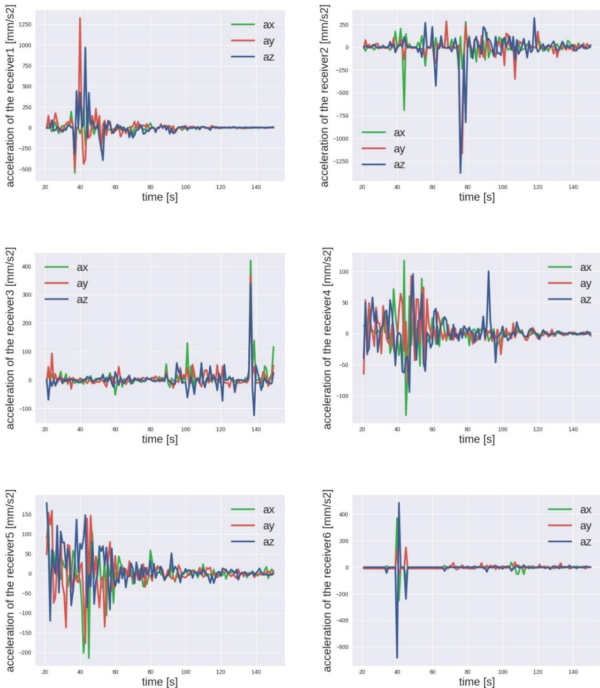
Fig. 57. Simulated acoustic signals generated by 220 m 3 of ice falling from the height of 3 m: acceleration readings from receivers 1 to 6 placed in water.
